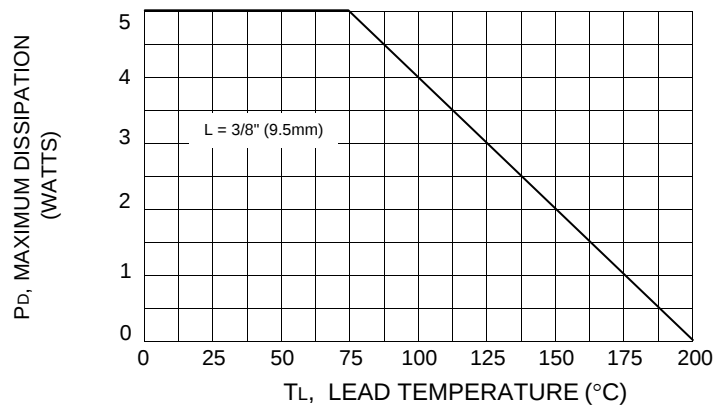
Fig 2. Typical Thermal Response L, Lead Length = 3/8 Inch
