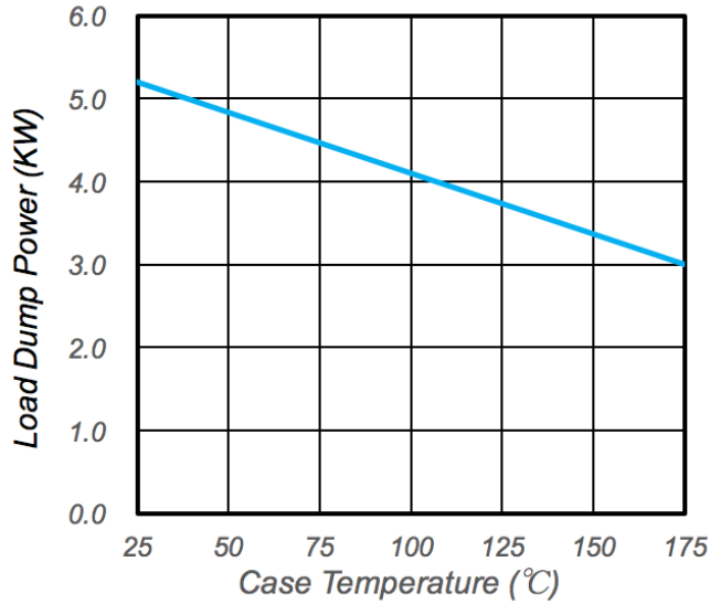
Fig.4 - Load Dump Power Characteristics (10ms Exponential Waveform)
