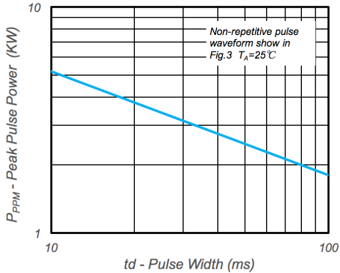
Fig.2 - Peak Pulse Power Rating
