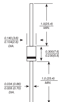
DO-15
